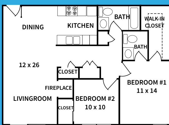
Third Floor w/Fireplace
